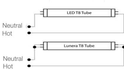
Correct Wiring
