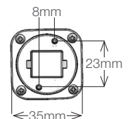
Bottom View 4-pin
